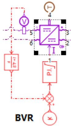
Figure 4 DC/DC converter with PID controller
